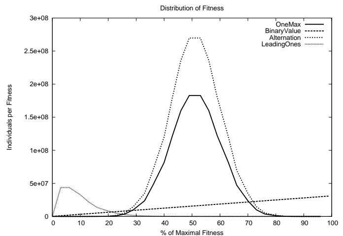
Figure 4: The frequency of individuals depending on the fitness of the individuals during a run of the EA_F . The data was obtained by taking the mean values of 25 runs on 30-bit individuals.
