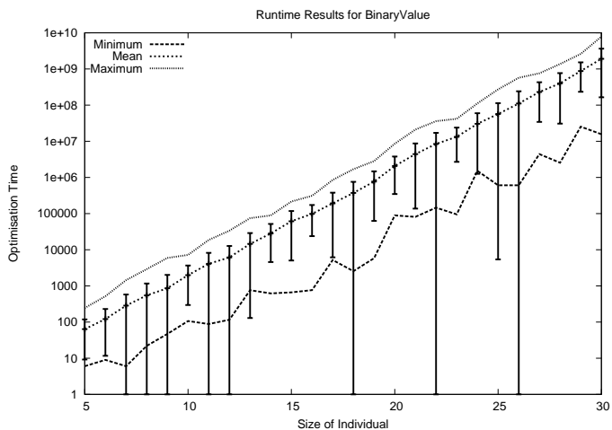
Figure 2: A closer look at the optimization time of the EA_F on BINARYVALUE. The minimum, maximum, and mean runtime (over 50 runs) is shown for individual of size 5 up to 30.
