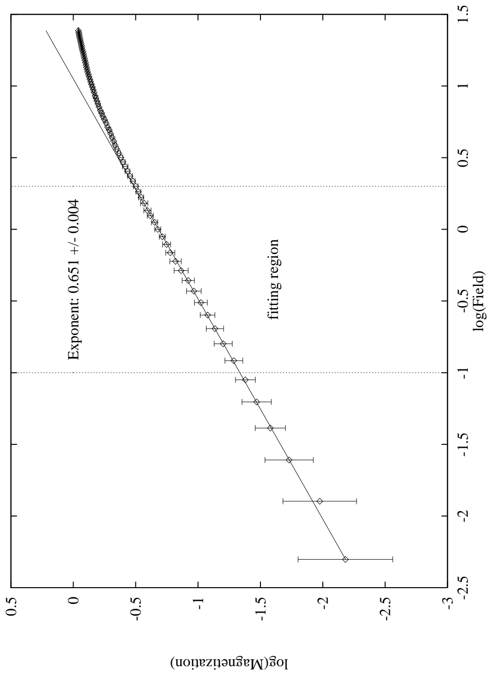
Fig. 3. Verifying a power law for the magnetization
