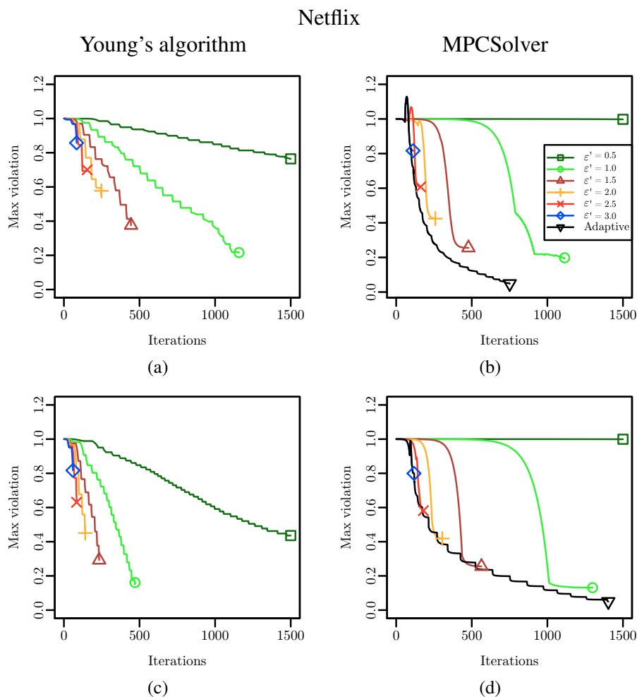
Figure 5.1: Efficiency of Young's algorithm and MPCSolver for 0.05-feasibility on Netflix (1x8)
