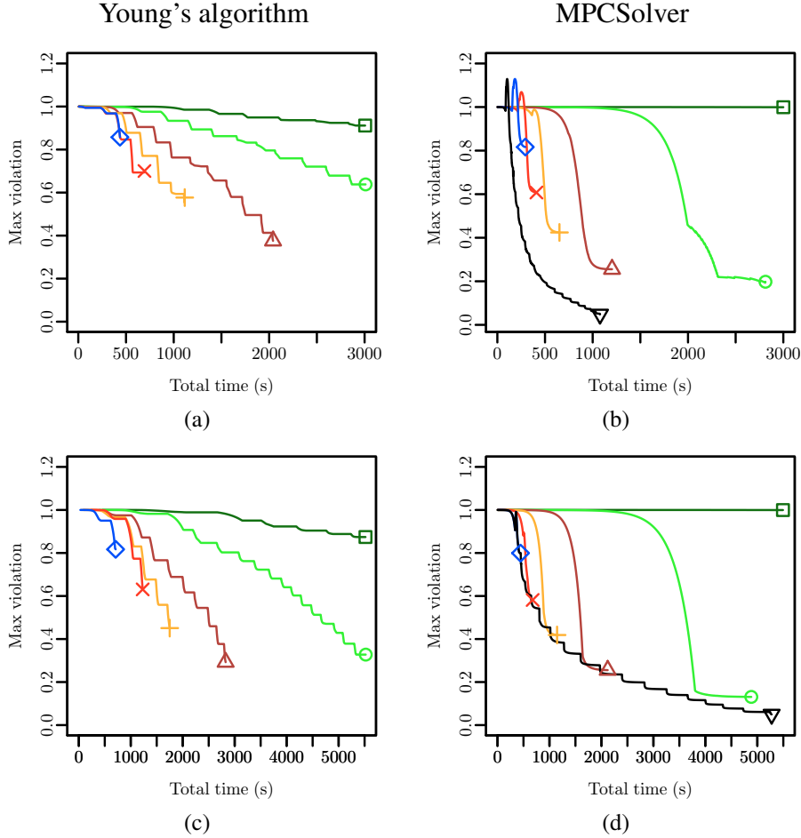
Figure 5.2: Efficiency of Young's algorithm and MPCSolver for 0.05-feasibility on KDD (1x8)
