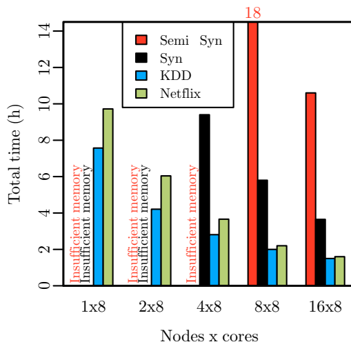
Figure 5.3: Scalability of DDRounding on different datasets
