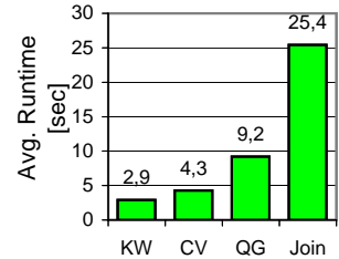
Figure 11: Avg. runtimes
