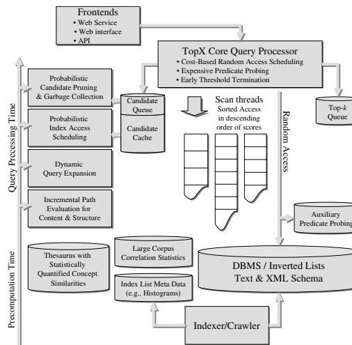
Figure 1: TopX Architecture
