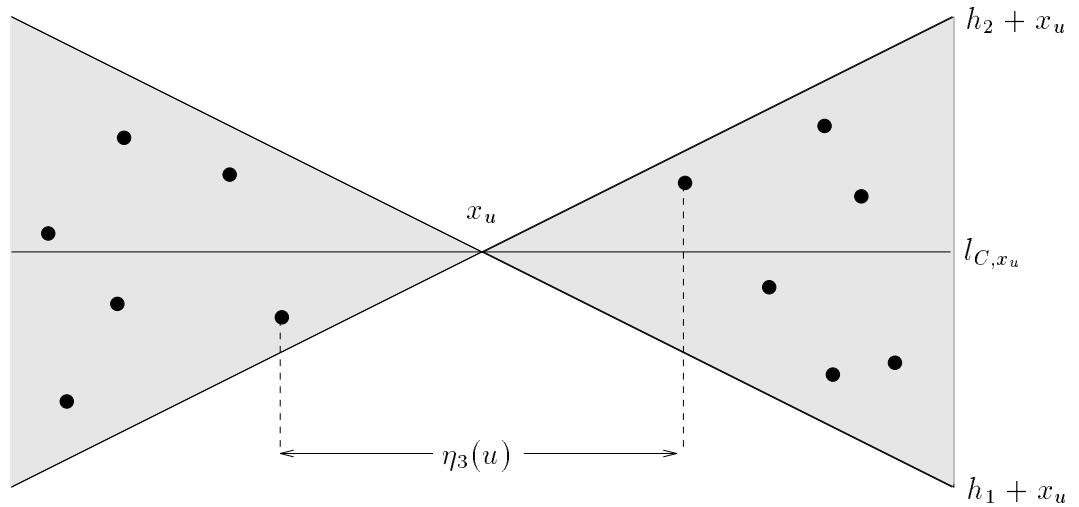
Figure 6: Illustration of the (d + 1) -layered data structure for d = 2 . The points in the cone C_{x_u} belong to the set S_{u,3}^+ ; those in the cone -C_{x_u} belong to S_{u,3}^- .
