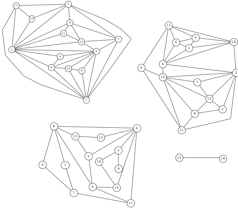
Figure 3: Decomposition of K_{14} with \text{THICK}_{JM}
