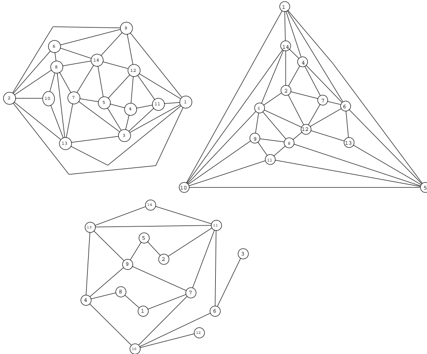
Figure 4: Decomposition of K_{14} with \text{THICK}_{JM} and a degree restriction of 6
