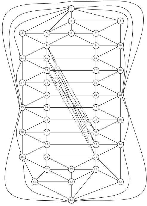
Figure 1: Graph G
