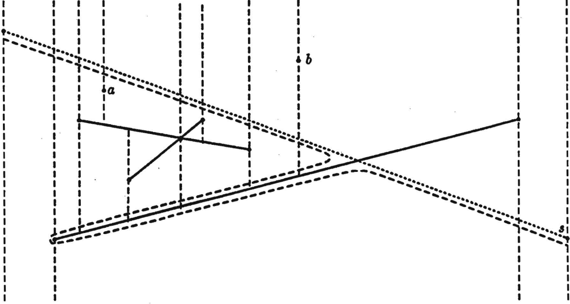
Figure 1: A trapezoidal decomposition T(R) for a subset R of three segments (shown solid) of a set S of five segments. The segment s (shown dotted) and the segment with endpoints a and b do not belong to R . When s is added to R the indicated walk (shown dashed) through T(R) is performed.
